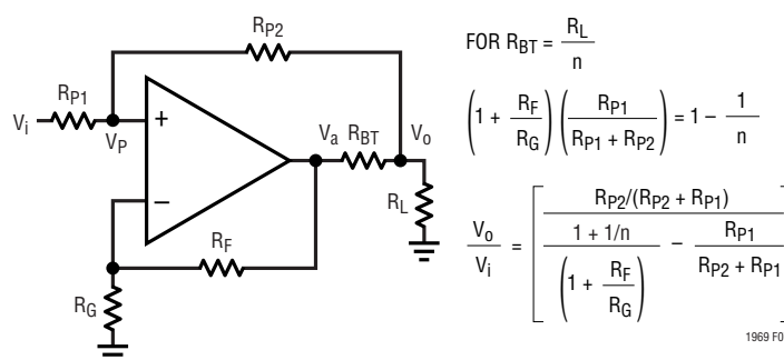
Figure 7. Back-Termination Using Positive Feedback
